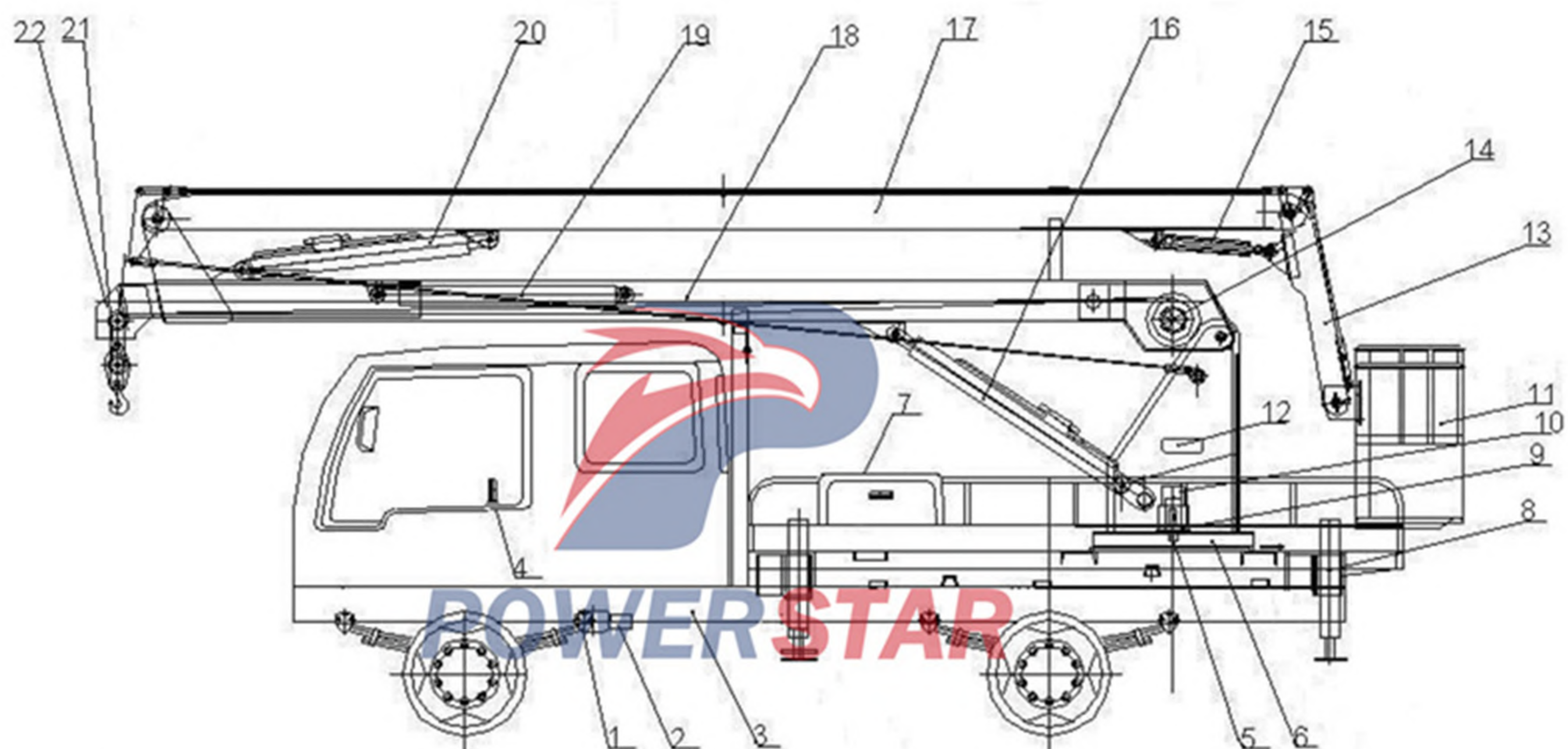
POWERSTAR Man Lifter Truck Technical Drawing:
